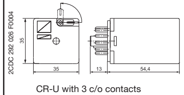
CR-U with 3 c/o contacts
