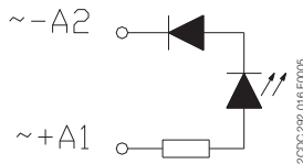
CR-P/M 62, CR-P/M 62E, CR-P/M 92, CR-P/M 92V, CR-P/M 62EV, CR-P/M 62V
