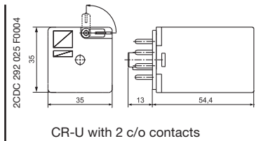
CR-U with 2 c/o contacts
