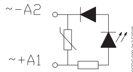
CR-P/M 62C, CR-P/M 62D, CR-P/M 92C, CR-P/M 92CV, CR-P/M 62DV, CR-P/M 62V
