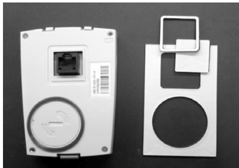
4. Separate square gasket from middle section.
