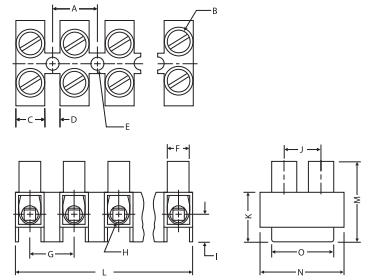
Dimensions mm
