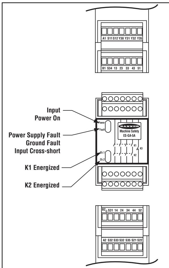
Figure 1. ES-...A-5A Status indicators and terminal locations
