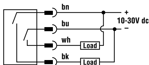
DC Sensors with Quick Disconnect (4-Pin Euro-Style)
