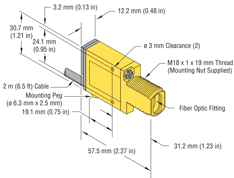
MINI-BEAM DC Sensor with Integral Cable
