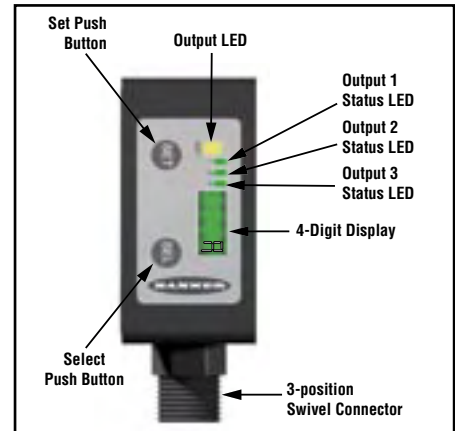
Figure 1. Sensor features
