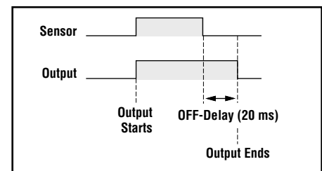
Figure 3. 20 ms OFF-delay (d_20): output continues for an interval after sensing stops (applies to all outputs)
