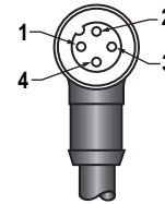
4-Pin Euro-Style Pinout (Cable Connector Shown)
