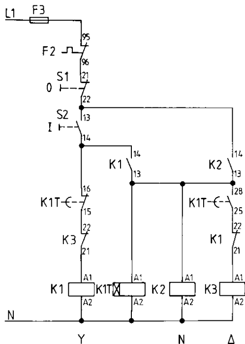
Diagram of control circuit
