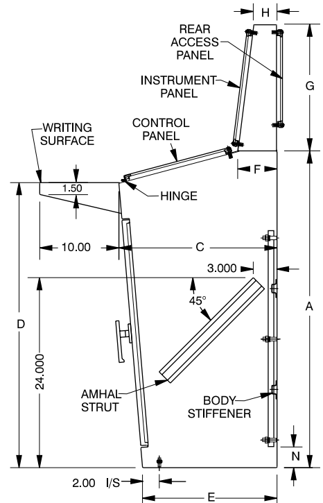
Section X-X
