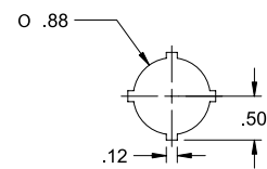
22.5mm Detail (1490M Series)
