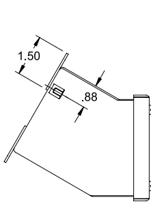
Side View 1490D1-D4 1490MD1-MD4
