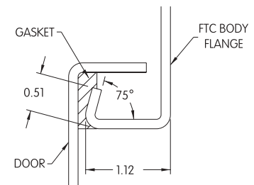
FTC Detail
