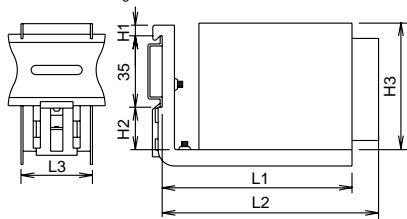
DIN-rail Mounting Bracket
