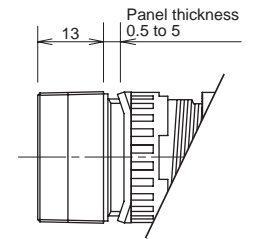
With Dustproof Cover Installed
