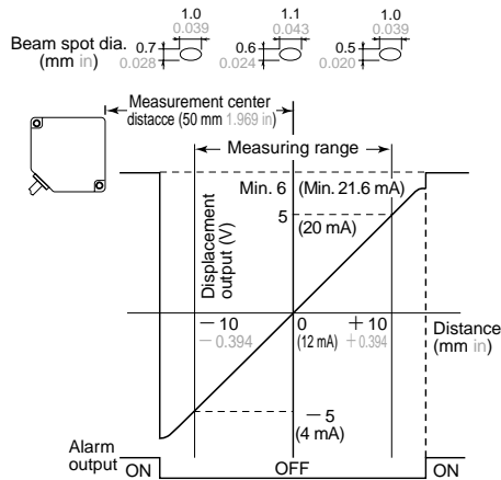
ANR1150 ANR1250
