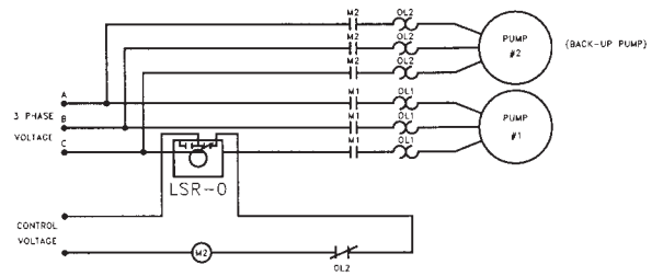
TYPICAL WIRING DIAGRAM FOR A MODEL LSR-0 FOR A DUPLEX PUMP SYSTEM
