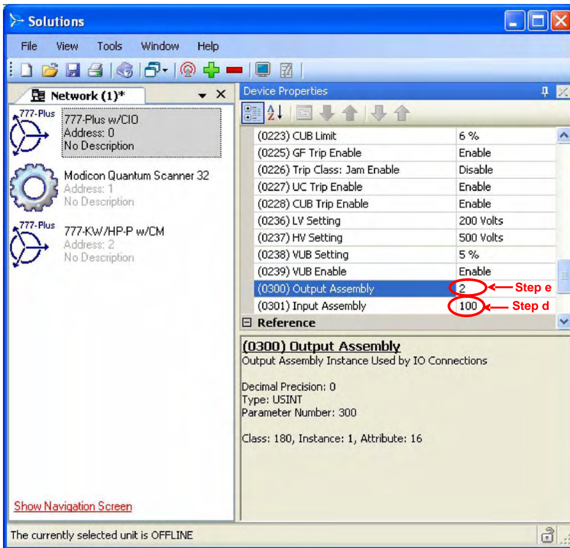
Figure 11-Variable Input Assembly
