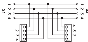
2-port Wiring Diagram
