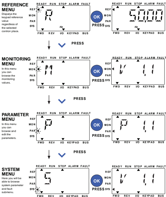
Figure 16: The main menu of Vacon 20
