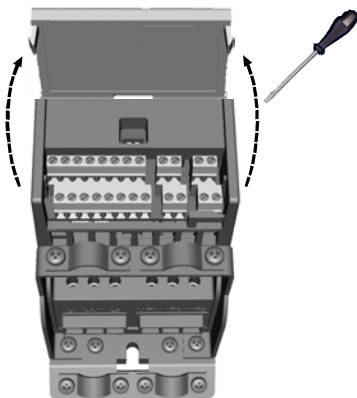
Figure 11: Open the lid MI1 - MI3
