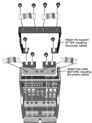
Figure 5: Attaching the PE-plate and API cable support, MI1 - MI3
