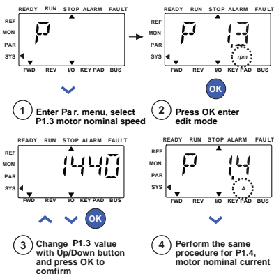
Figure 17: Vacon 20 startup wizard (standard application)
