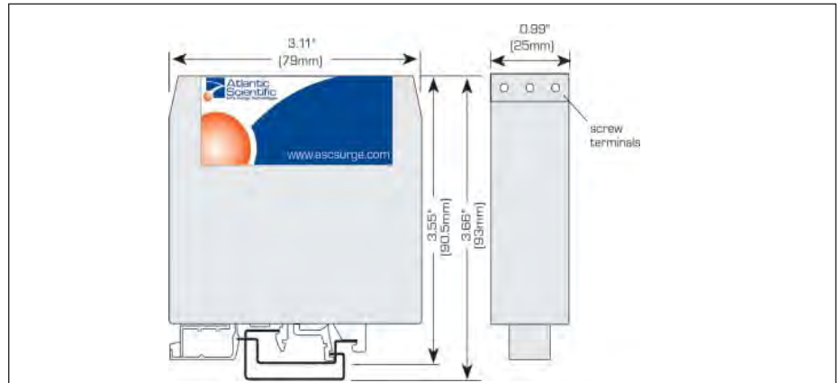
Figure 1 Dimensions
