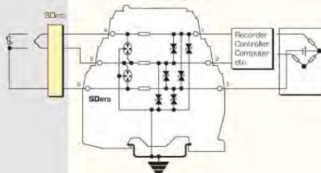
3-wire RTDs
