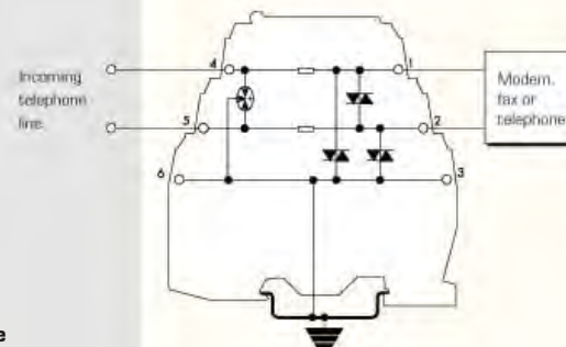
Telecom line
