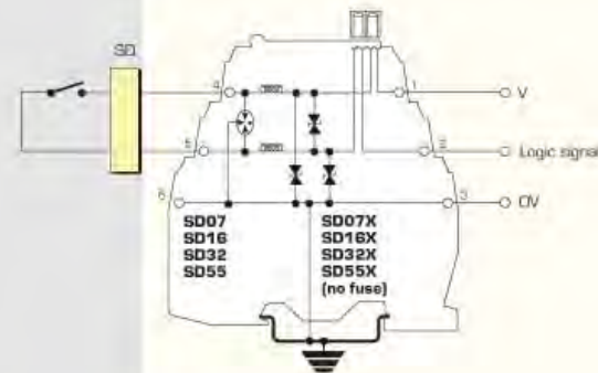
Switches
