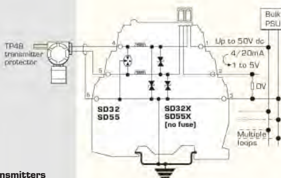
2-wire transmitters
