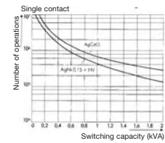
Contact service life under ohmic load
